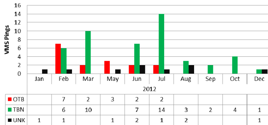
2012 UK activity by gear per month
