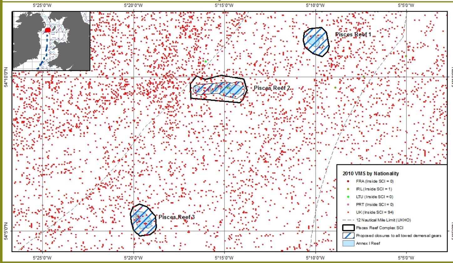
Figure 3: VMS reports from 2010 indicating all fishing activity in the Pisces Reef Complex SCI by Nationality.
