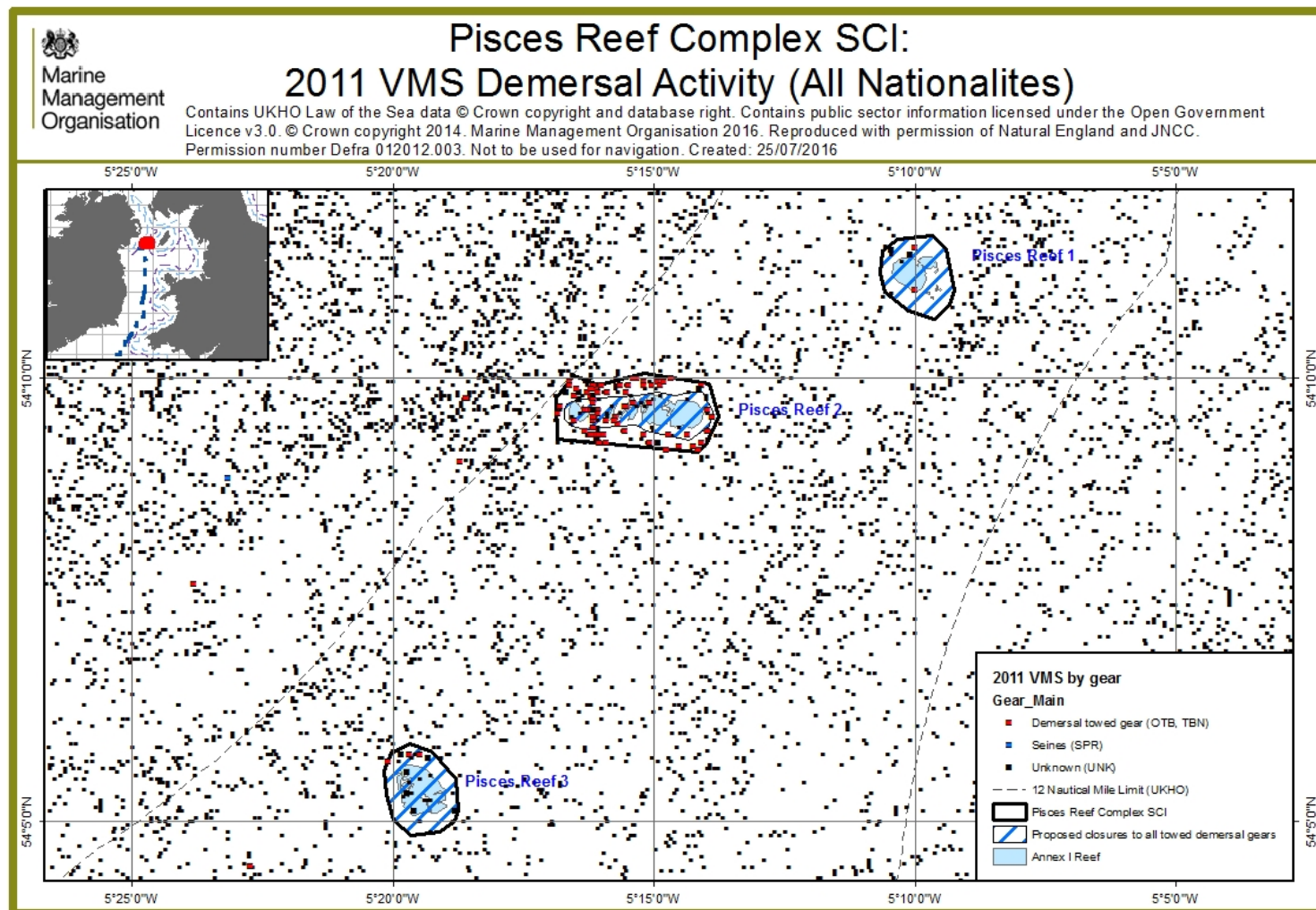
Figure 10: VMS reports from 2011 indicating demersal fishing activity in the Pisces Reef Complex SCI by gear type.
