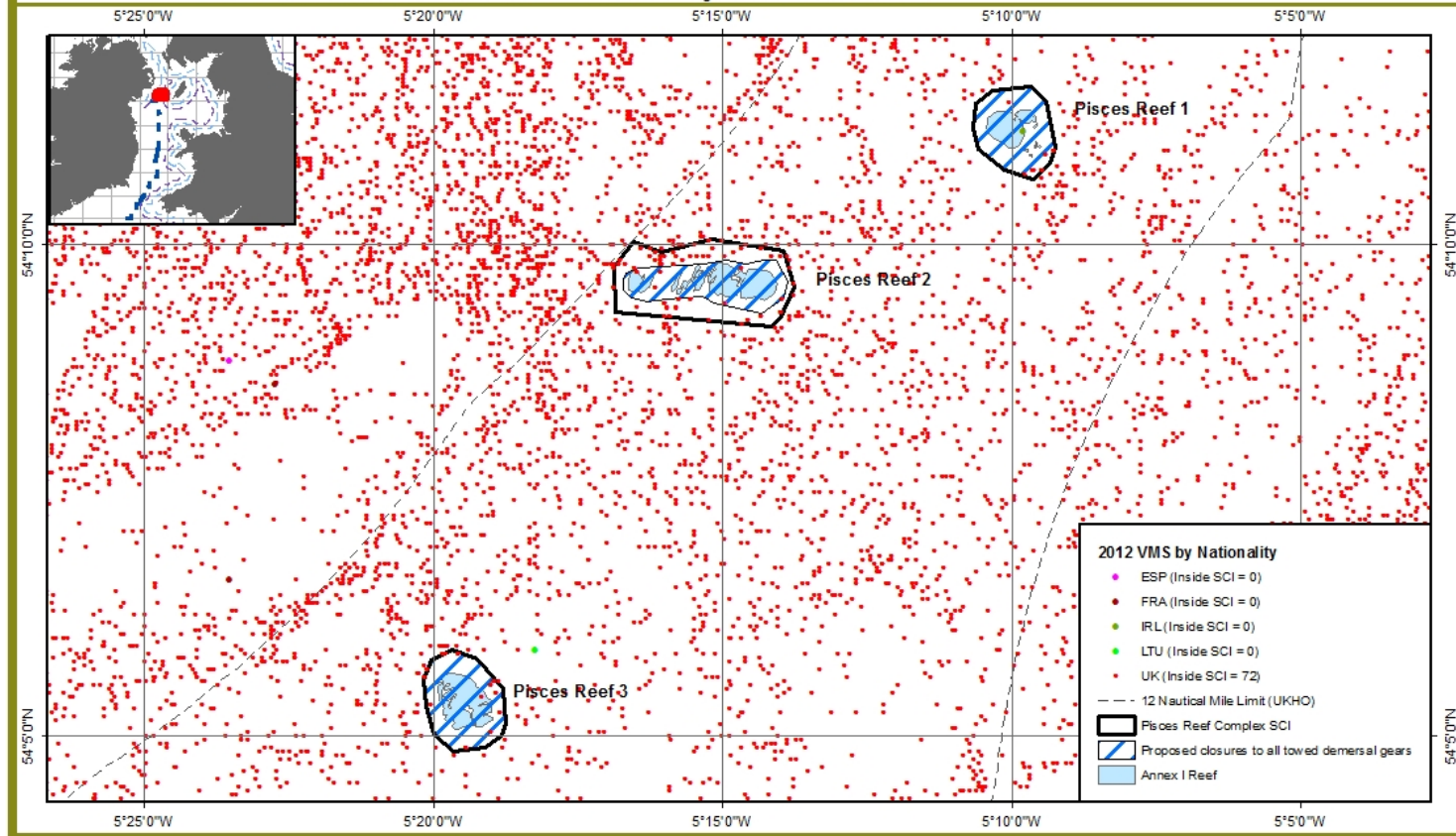
Figure 5: VMS reports from 2012 indicating all fishing activity in the Pisces Reef Complex SCI by Nationality.
