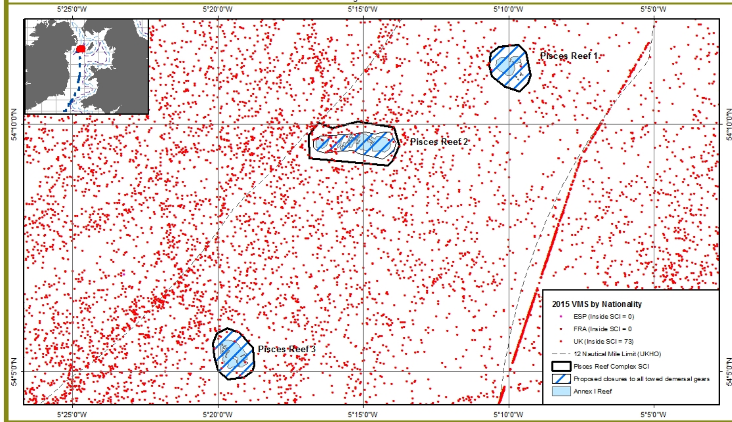
Figure 8: VMS reports from 2015 indicating all fishing activity in the Pisces Reef Complex SCI by Nationality.
