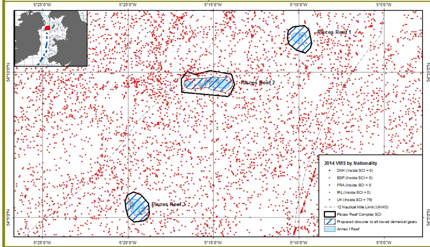
Figure 7: VMS reports from 2014 indicating all fishing activity in the Pisces Reef Complex SCI by Nationality.
