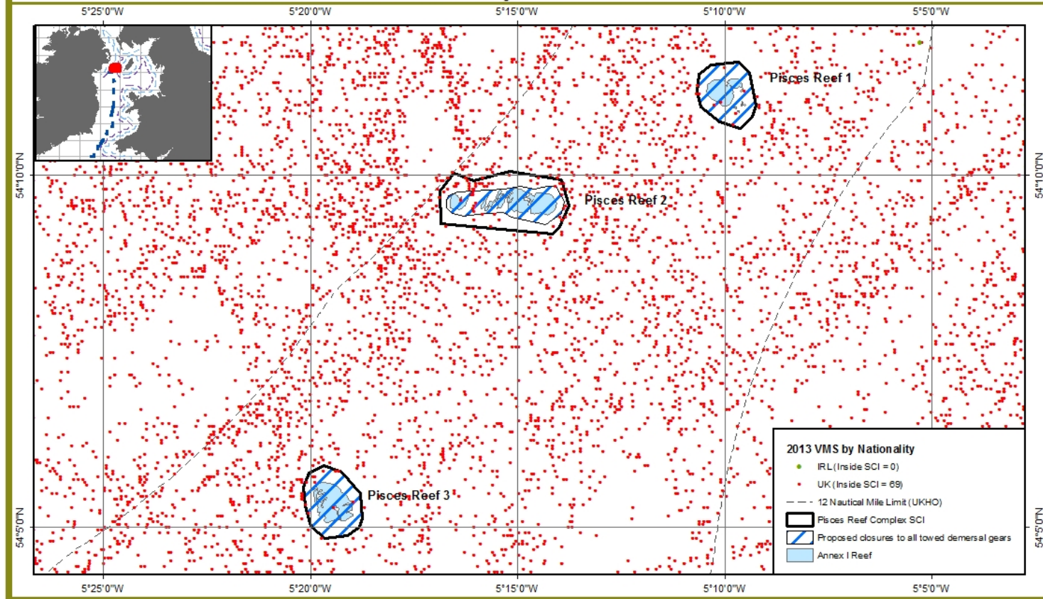
Figure 6: VMS reports from 2013 indicating all fishing activity in the Pisces Reef Complex SCI by Nationality.
