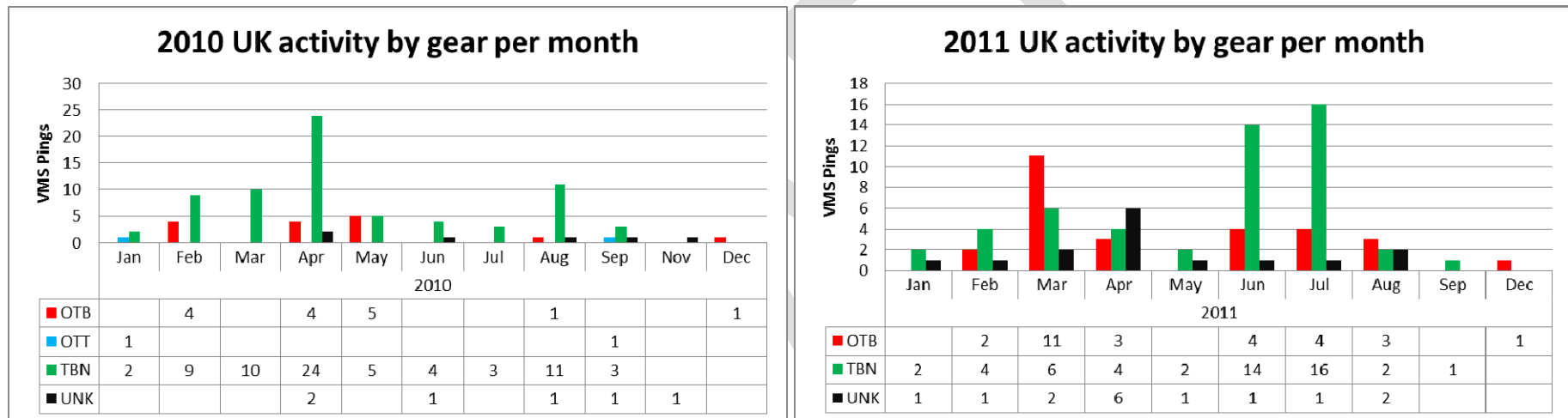
Chart 6.1: UK seasonal fishing activity (all gears) in Pisces Reef Complex SCI.
