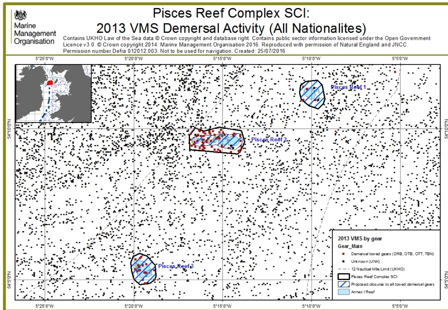
Figure 12: VMS reports from 2013 indicating demersal fishing activity in the Pisces Reef Complex SCI by gear type.
