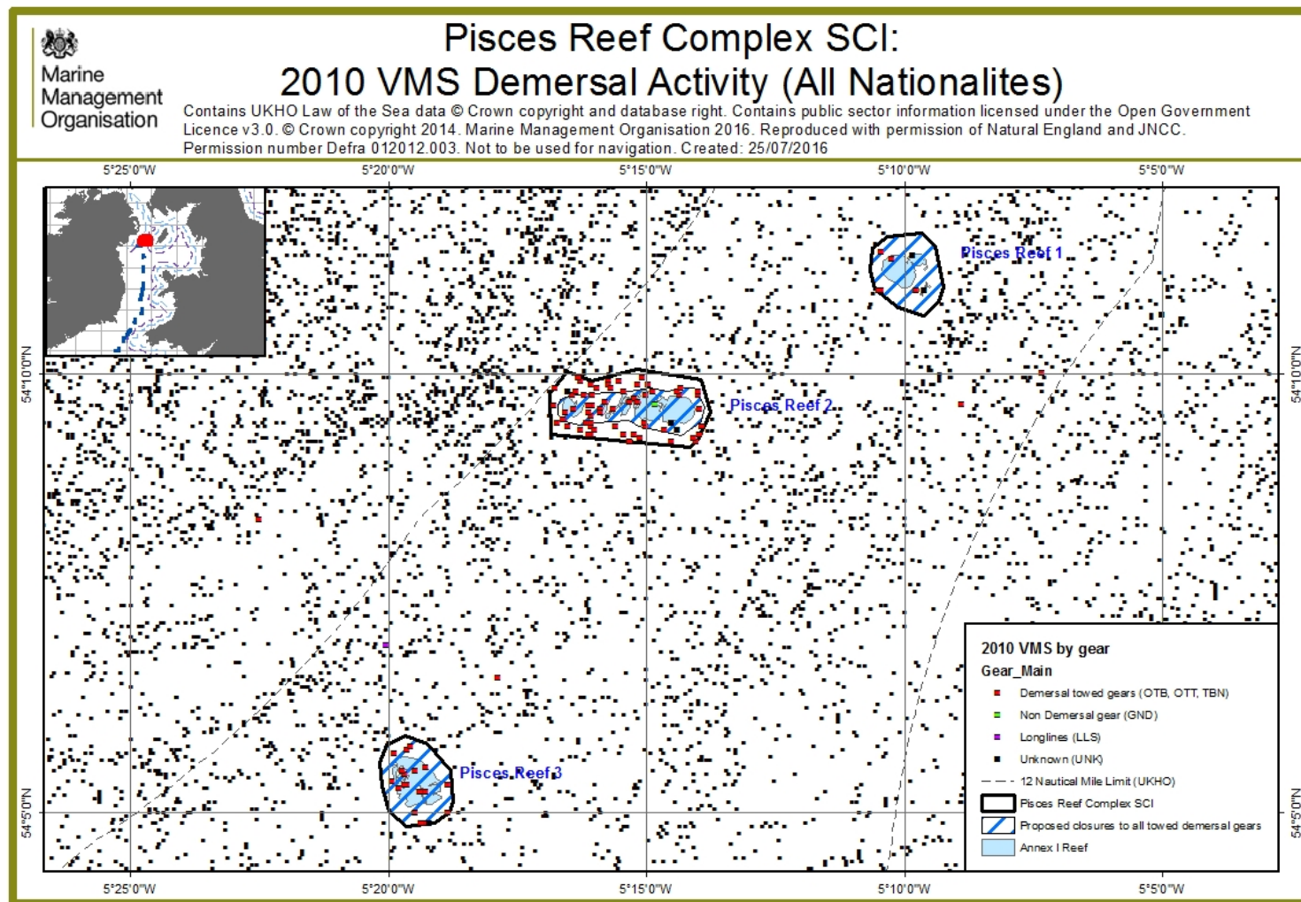
Figure 9: VMS reports from 2010 indicating demersal fishing activity in the Pisces Reef Complex SCI by gear type.
