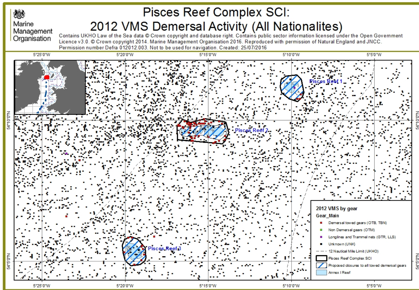
Figure 11: VMS reports from 2012 indicating demersal fishing activity in the Pisces Reef Complex SCI by gear type.
