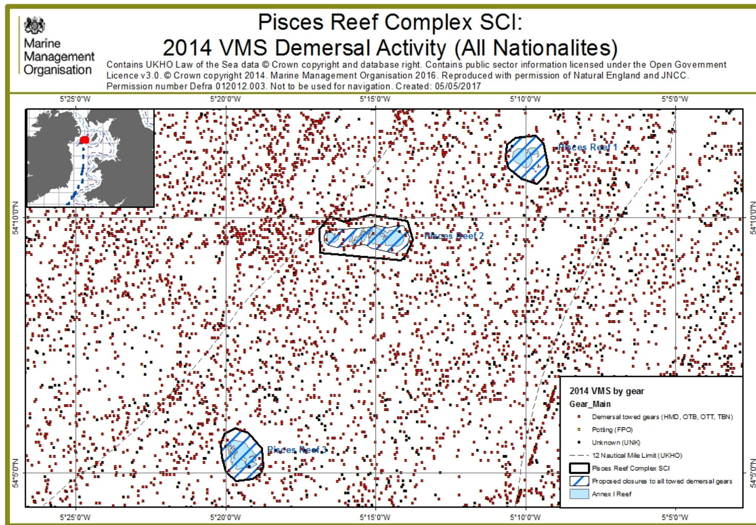
Figure 13: VMS reports from 2014 indicating demersal fishing activity in the Pisces Reef Complex SCI by gear type.
