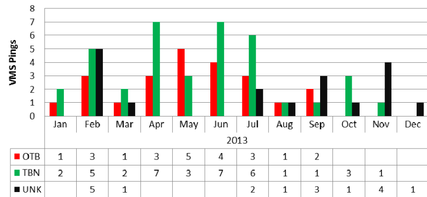
2013 UK activity by gear per month
