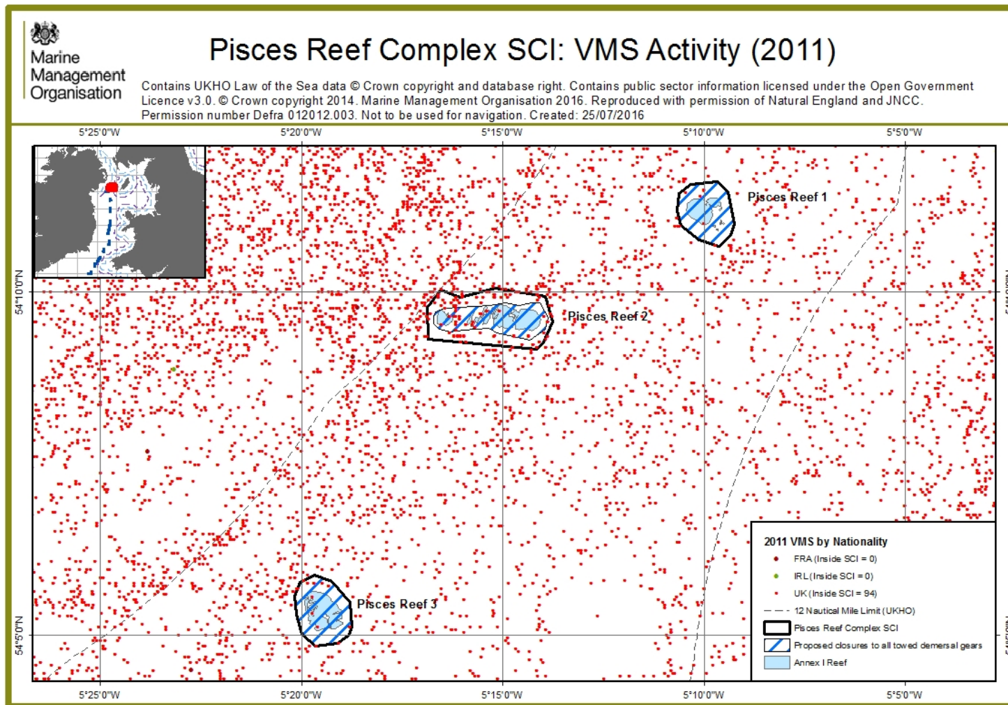
Figure 4: VMS reports from 2011 indicating all fishing activity in the Pisces Reef Complex SCI by Nationality.
