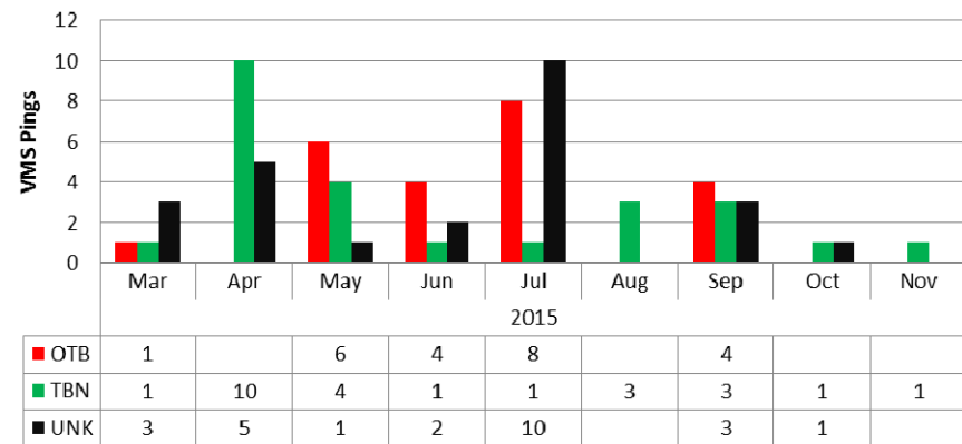
2015 UK activity by gear per month
